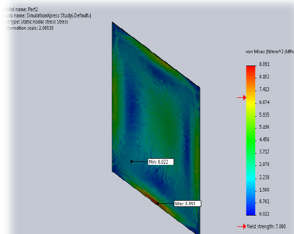
Fig.5: Simulation X stress Study-Stress-Stress
