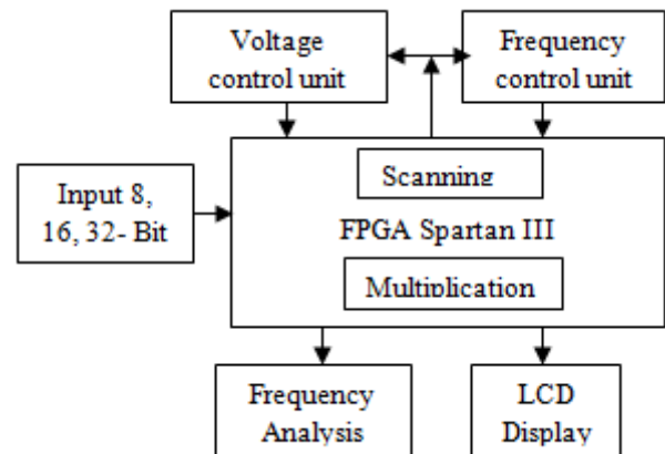
Fig. 1: Architecture of multiplier system
