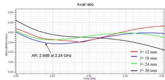
Fig. 6: Axial ratio for different segment length (l)
