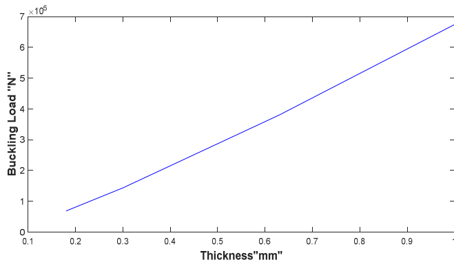
Fig.6:Effect of thickness on buckling load
