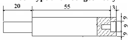
Figure. 3.1(a): Emboss Type electrodes without Flushing hole in Brass & Copper Electrodes.
