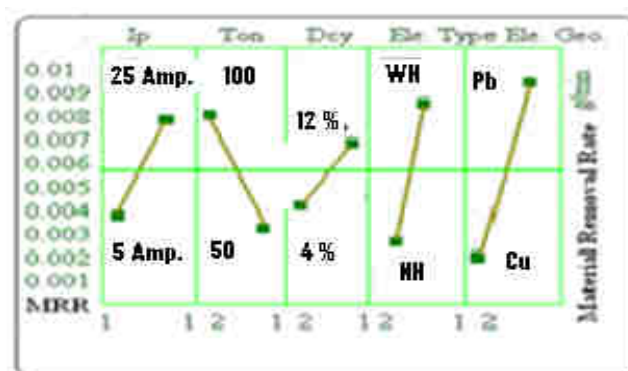
Fig.3.3: Main effects plot for MRR
