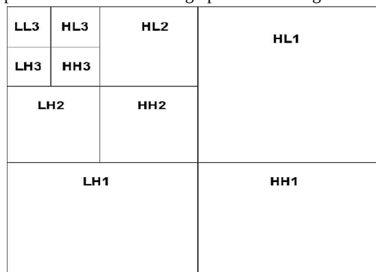
Fig. 3:Discrete Wavelet Transform
