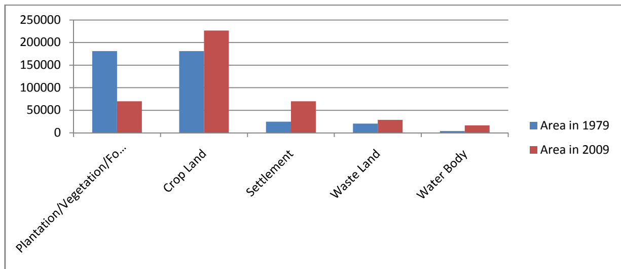
Fig. 3: Graph depicting Land use Land cover area of 1977 Ind 2009.
