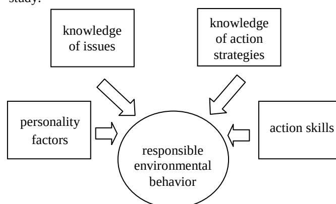
Fig.1:Theoretical Paradigm
