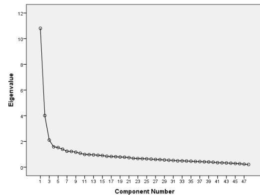
Fig.2:Scree Plot
