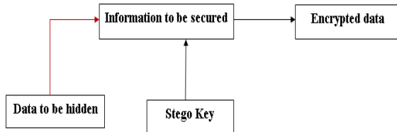
Fig.2: Steganography process
