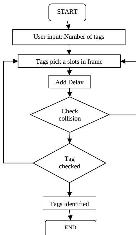
Fig.3: Flowchart of simulation
