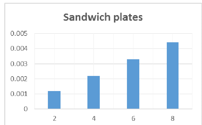
Fig. 4.3 No. of Plates Vs Damping of Sandwich plates
