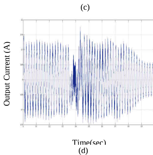
Fig. 6 (a) Speed and load Torque Response (b) Stator and Rotor Current (c) Input Current (d) Output Current at Abnormal input supply
