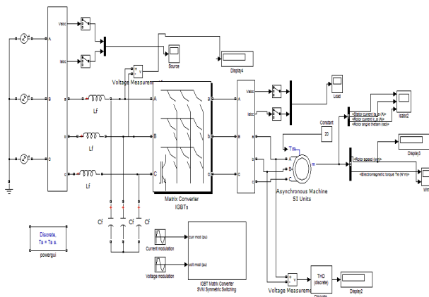
Fig. 4: SVM Based simulation model for induction motor fed by a three phase matrix converter
