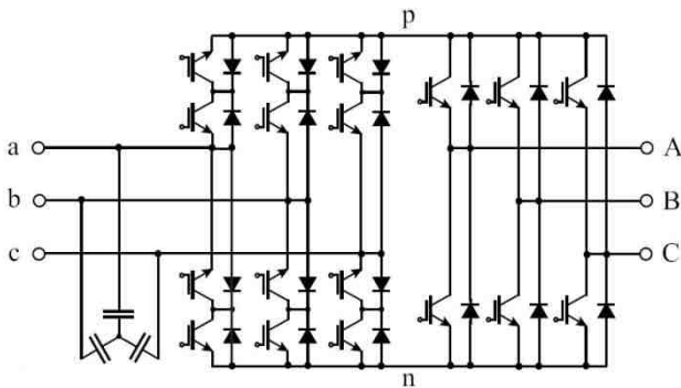
Fig. 2: Indirect Matrix Converter
