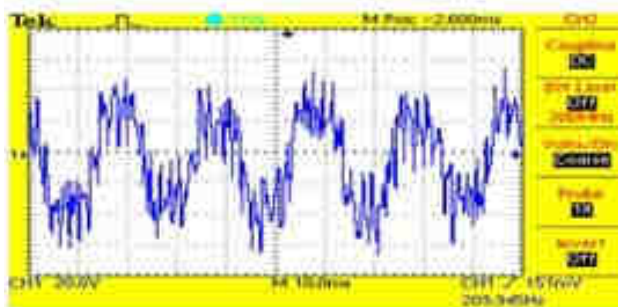
Fig. 8: Output line current at 30 Hz.
