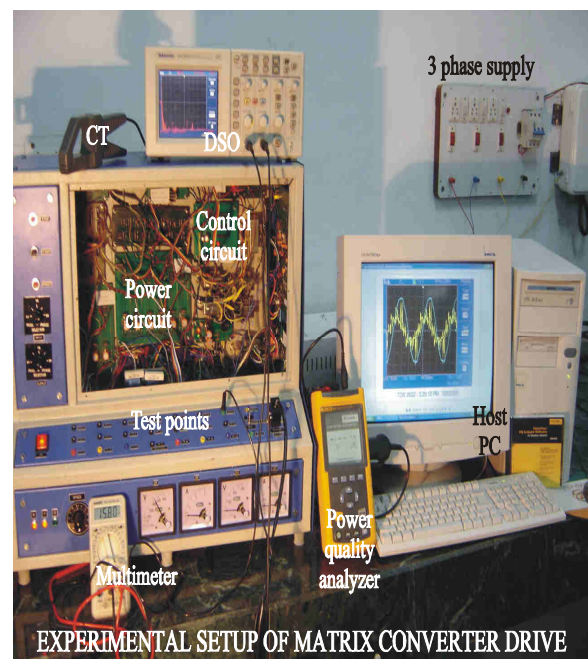
Fig. 5: Experimental set-up of the matrix converter drive system
