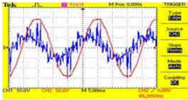
Fig. 7: Input & Output phase voltage at 30 Hz.
