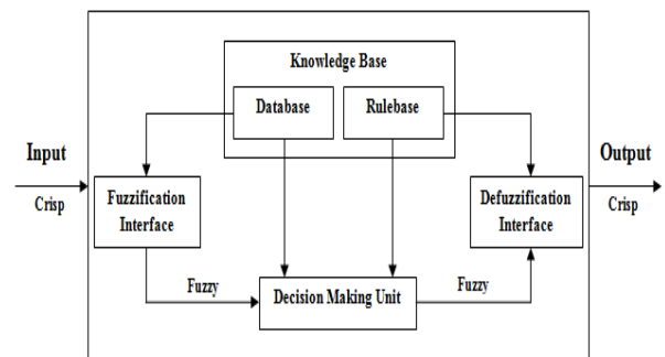
Fig 1: Fuzzy inference system
