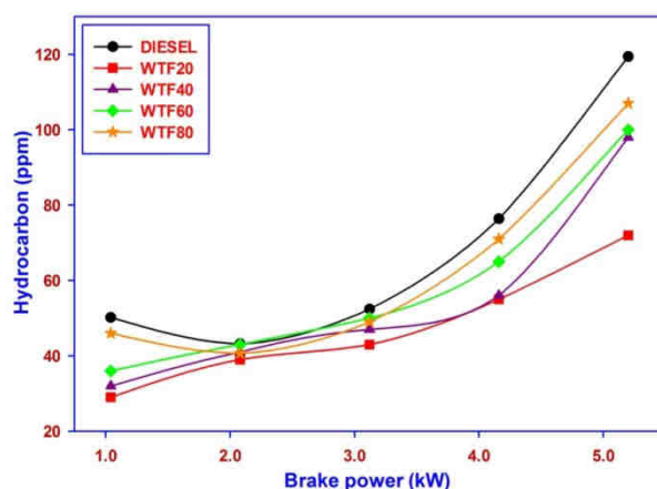
Fig. 9 Hydrocarbon against brake power
