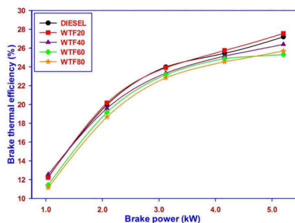
Fig. 4 Brake thermal efficiency against brake power
