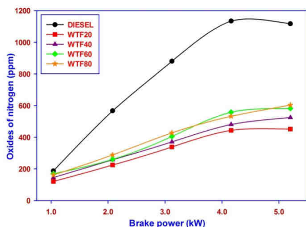
Fig. 6 Oxides of nitrogen against brake power
