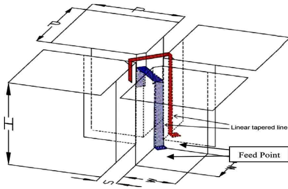
Fig.1. Geometry of I shaped feed
