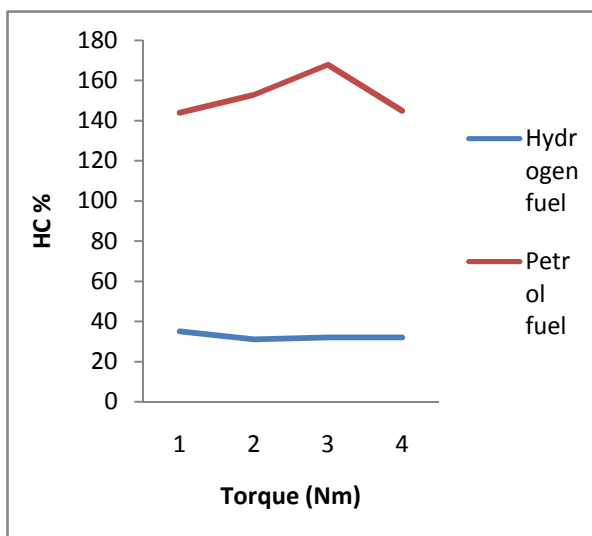
Fig. 7 Hydrocarbon Emission against Torque
