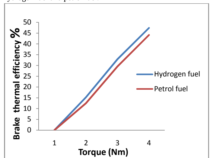
Fig. 5 Brake Thermal Efficiency against Torque
