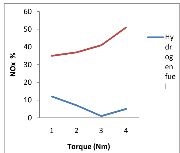
Fig. 9 Oxides of nitrogen against Torque
