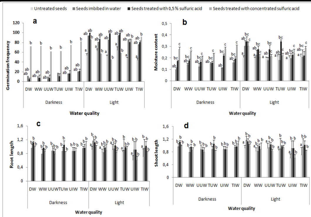
Fig. 3: Effects of water quality, incubation condition (light / darkness) and seeds pretreatment on (a) germination rate, (b) moisture content, (c) root and (d) shoot lengths of Lawsonia inermis seeds.
