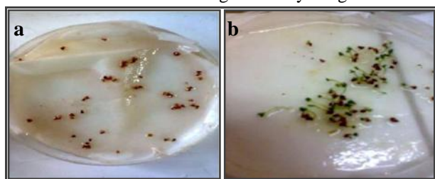
Fig. 2: (a) Lawsonia inermis seeds put in germination; (b) Seeds after 7 days of germination in the light.
