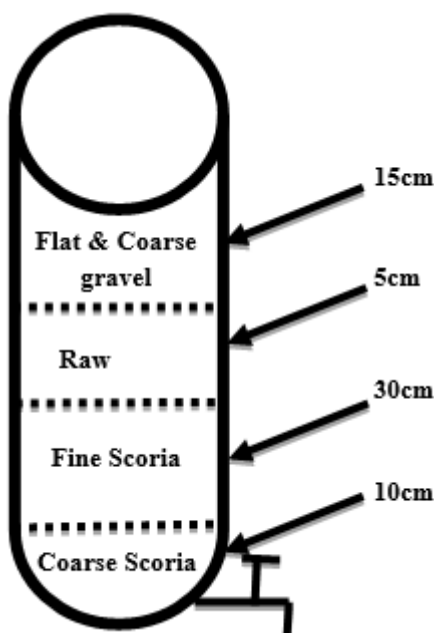
Fig. 2: Schematic layout of the Tanker Components of scoria filter
