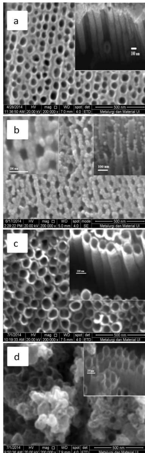
Figure 1. FESEM image of top surface TNPs-NTAs (a). top surface CdS/TNPs-NTAs and high magnification image, (b). top surface TNTAs, (c). top surface CdS/TNTAs and (d). with inset are cross section views
