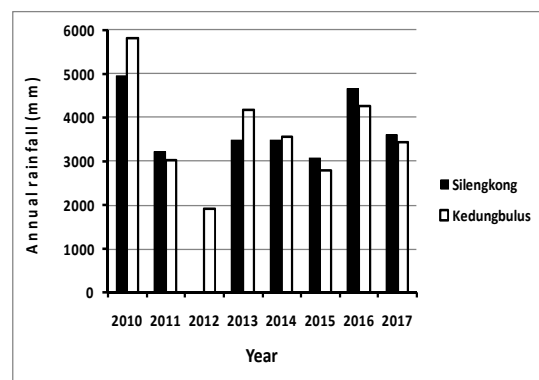
Figure 2. Annual rainfall at two stations of the study area
