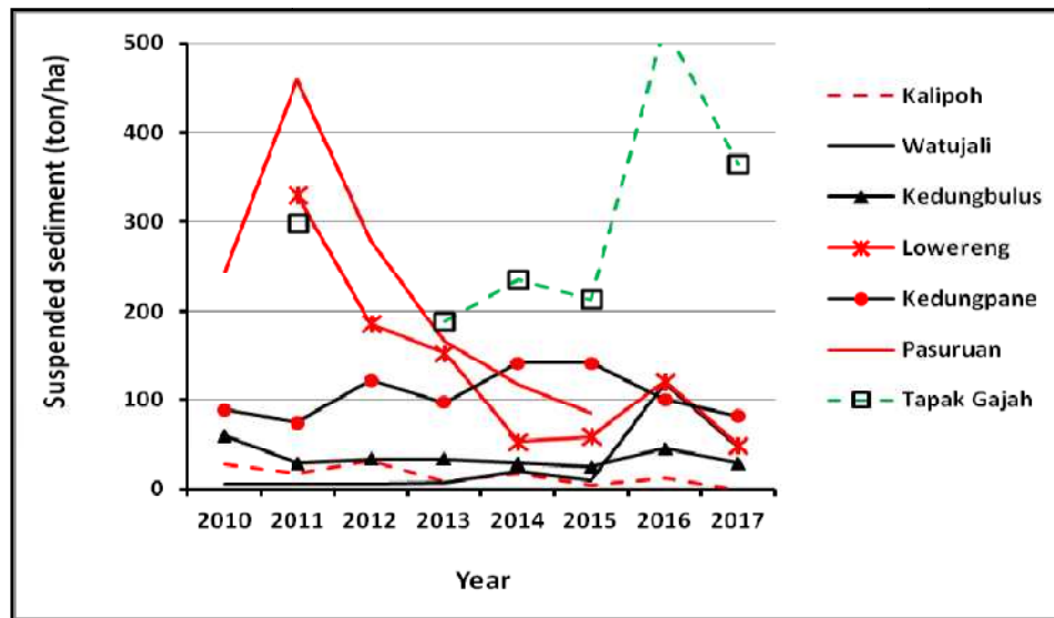
Figure 6. Annual suspended sediment of the observed catchments
