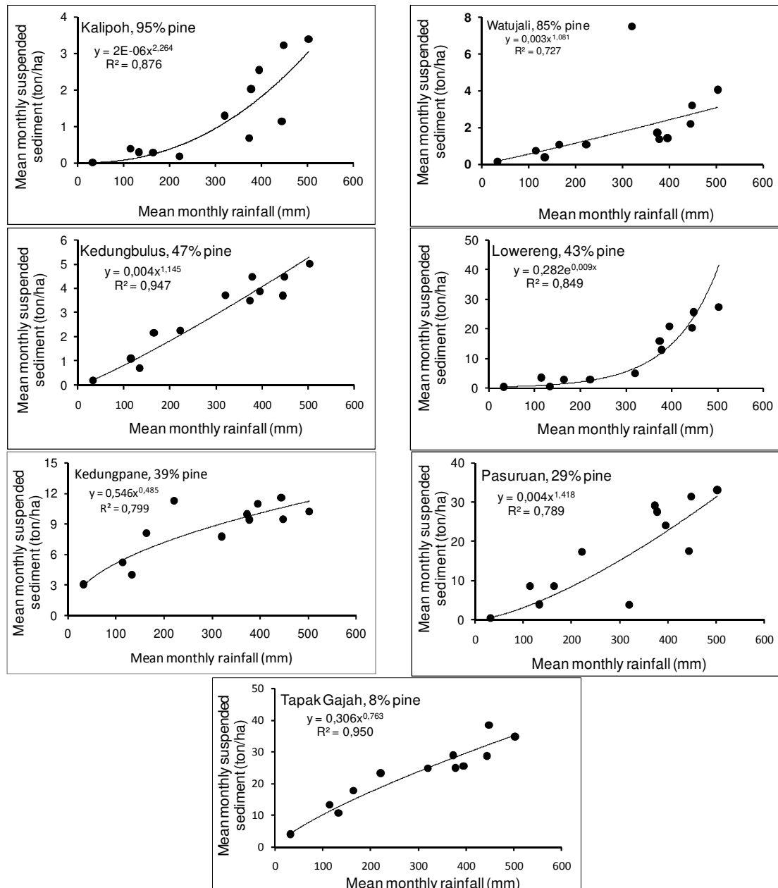
Figure 4. The relationship of mean monthly rainfall (mm) and mean monthly suspended sediment (t/ha) Source: Primary data analysis
