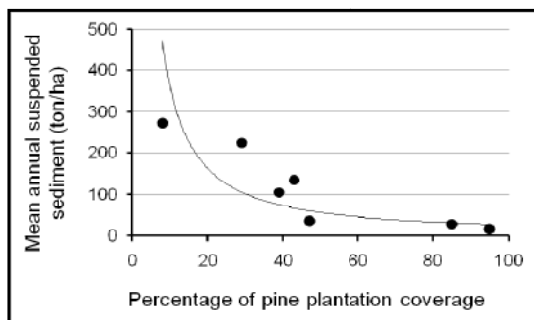
Figure 7. The scatter plot of plantation area vs mean annual suspended sediment
