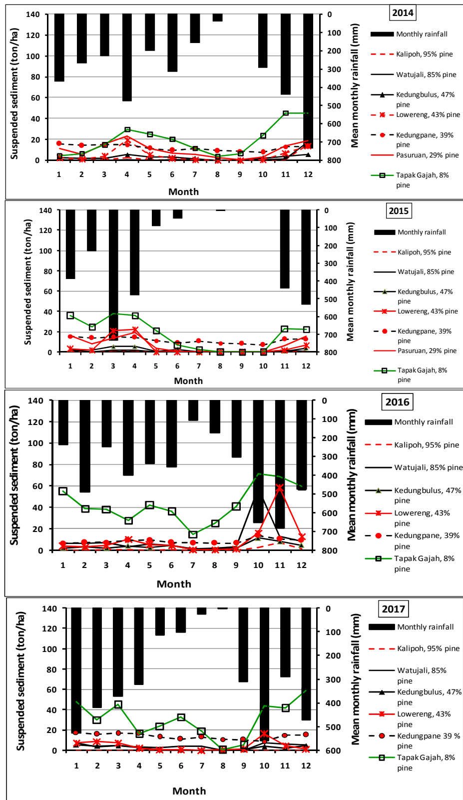
Figure 5. Temporal distribution of monthly rainfall and suspended sediment of the catchments Source: Primary data analysis
