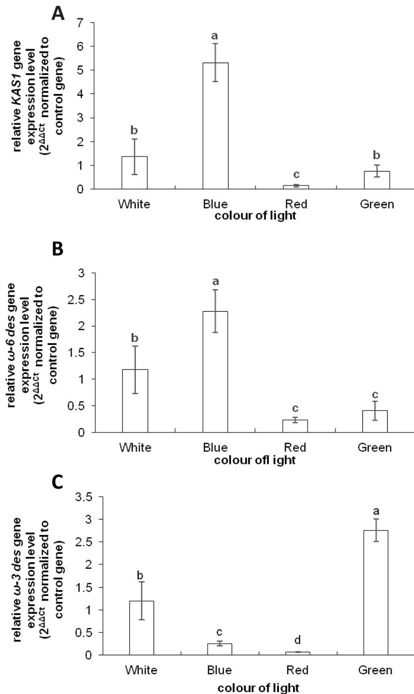
Figure 5 Effect of light color on mean fold change in relative expression of: (A) KAS-1 ; (B) \omega -6 FAD; and (C) \omega -3 FAD of Chlorella strain KS-MA2 (mean \pm SD; n=3)
