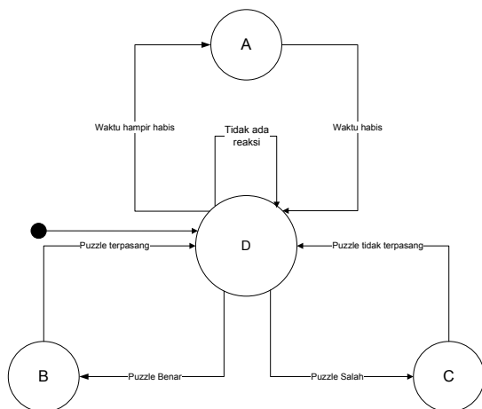
Gambar 5. Rancangan FSM ( Finite State Machine ).
