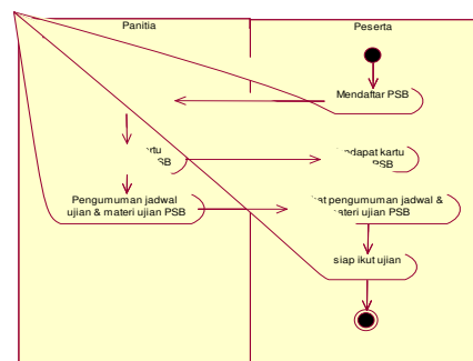
Gambar 6. Activity Diagram Daftar PSB
