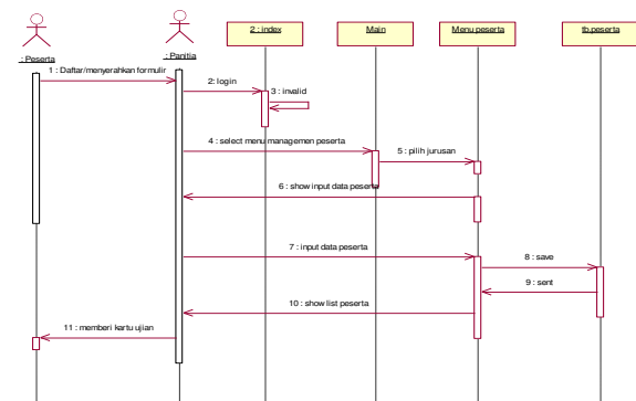
Gambar 17. Diagram Sequence Daftar PSB
