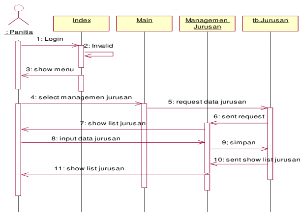
Gambar 16. Diagram Sequence Jurusan
