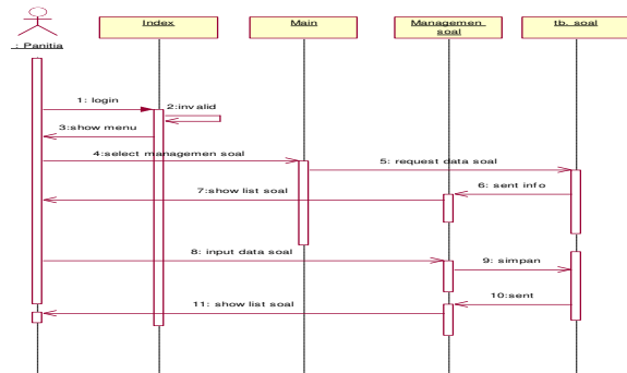
Gambar 15. Diagram Sequence Soal
