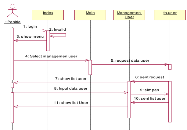
Gambar 14. Diagram Sequence User
