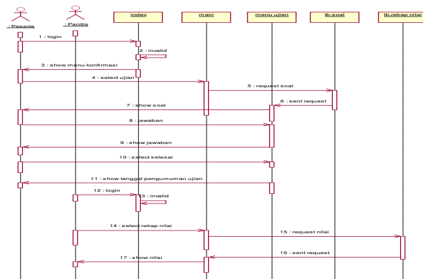
Gambar 18. Diagram Sequence Ujian
