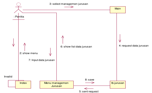
Gambar 21. Diagram collaboration jurusan
