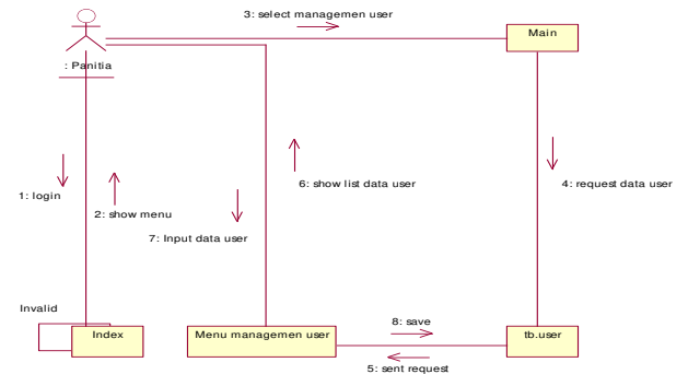
Gambar 19. Diagram collaboration User
