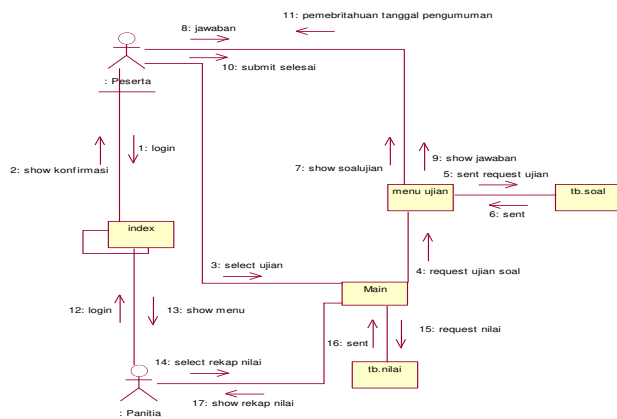
Gambar 23. Diagram collaboration Ujian
