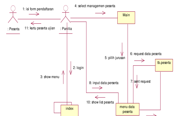
Gambar 22. Diagram collaboration Daftar PSB
