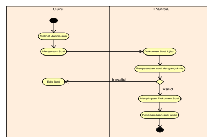
Gambar 5. Activity Diagram Soal
