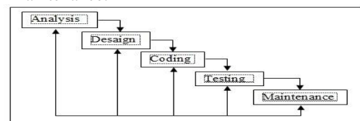
Gambar 1. Metode WaterFall
