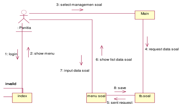
Gambar 20. Diagram collaboration soal
