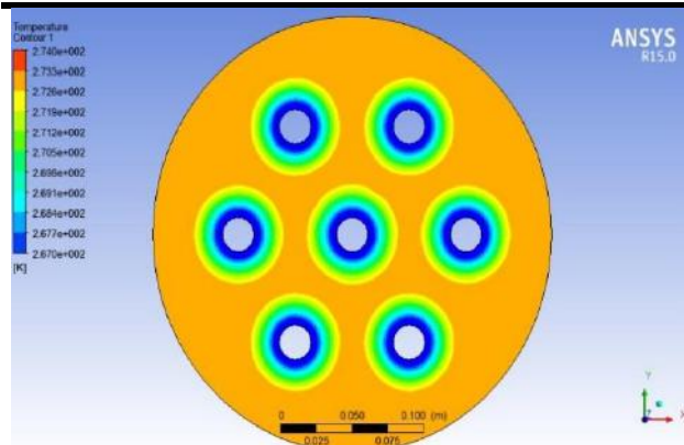
Fig.12: Temperature distribution along the diameter of the copper pipes in a storage tank.
