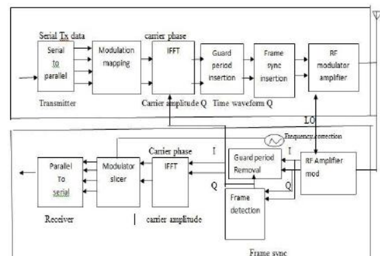
Fig.1.1: OFDM Transceiver System
