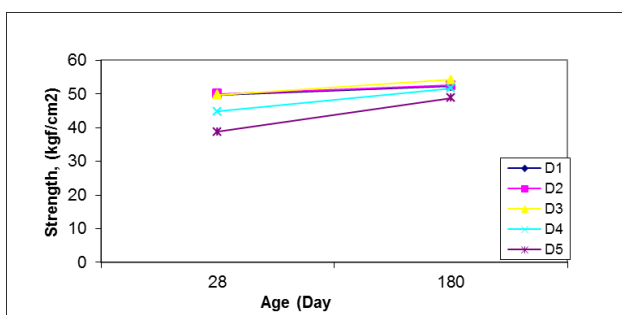
Fig.4: Splitting tensile strength test results (S/B=0,50 and 350 dose)
