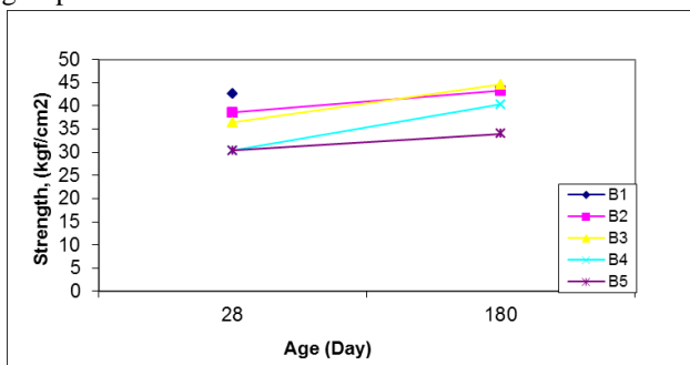
Fig.3: Splitting tensile strength test results (S/B=0,60 and 350 dose)
