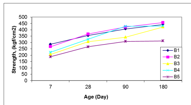
Fig.1: Compressive Strength test results (W/B=0,60 and 350 dose)
