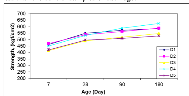
Fig.2: Compressive Strength test results (W/B=0,50 and 350 dose)
