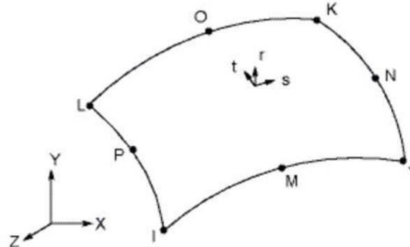
Fig. 3: 8-point quadratic elements for ANSYS
