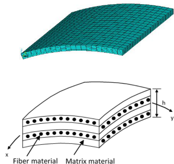
Fig. 1: Fiber and matrix materials in laminated composite shell
