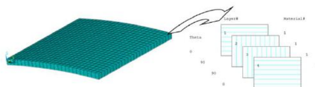
Fig. 2.b: Layered sequence for cylindrical shallow shell [12]
