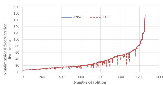
Fig. 4: Comparison of Ansys and SDSST Model Results for each of all data set
