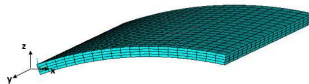
Fig. 2.a: Cylindrical shallow shell [12]
