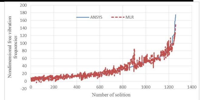
Fig. 5: Comparison of Ansys and MLR Model Results for each of all data set
