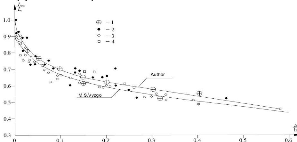
Fig.2: Diagram \frac{L_{frik}}{L_0} = f\left(\frac{\Delta}{h_2}\right) .
