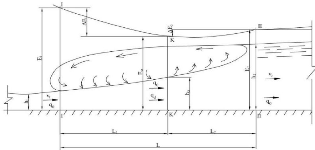
Fig.1: Calculation diagram
