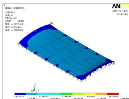
Fig. 9: Field of von mises stress of the shell at time t = 0.021s
