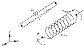
Fig. 4: COMBIN14 Geometry [8]
