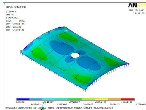
Fig. 13: Field of von mises stress of the shell at time t = 0.021s
