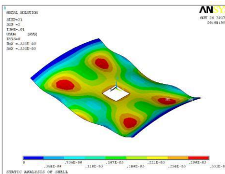
Fig. 24: The overall transposition field of the structure at time t = 0.01s
