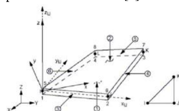
Fig. 2: SHELL63 Geometry
