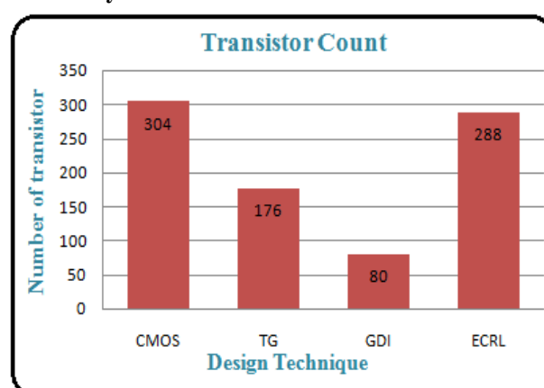
Fig.4.2.1 Transistor count for CLA using Different design technique
