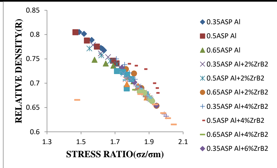
Fig. 12: Relative density Vs Stress ratio( \sigma_z/\sigma_m ).
