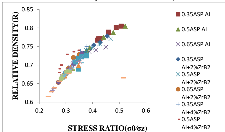
Fig. 11: Relative density Vs Stress ratio( \sigma\theta/\sigma_z ).
