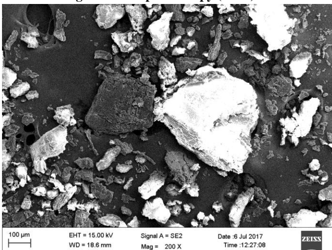
Fig.2: Before Adsorption
