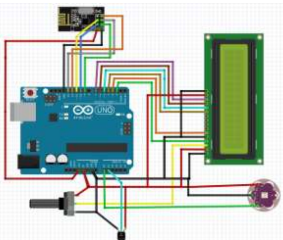
Fig. 4.1: Circuit Diagram of Transmitter section
