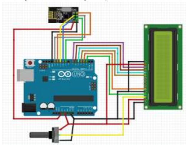
Fig. 4.2: Circuit Diagram of Receiver Section
