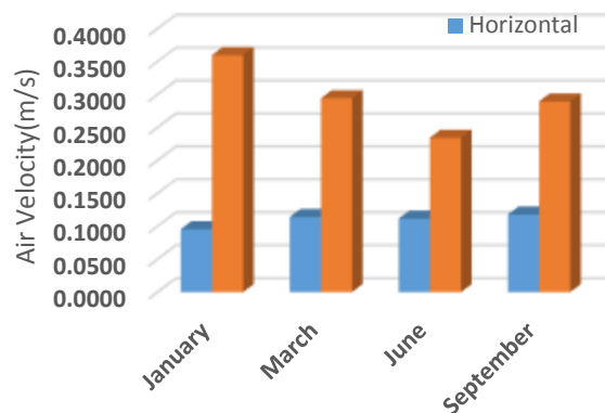
Fig.4.6: Design comparisons for solar chimney at SC-out measuring location
