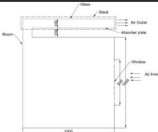
Fig.4.2: Line Diagram of Horizontal Solar Chimney
