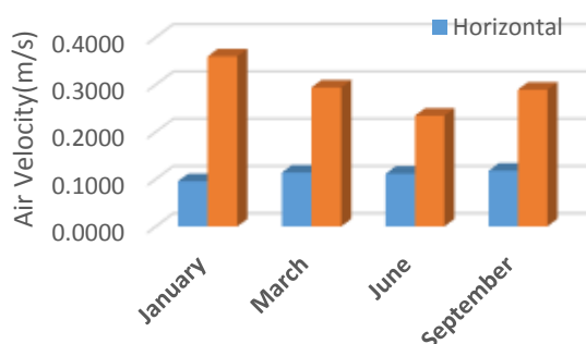
Fig.4.3: Design comparisons for solar chimney at R-500 measuring location
