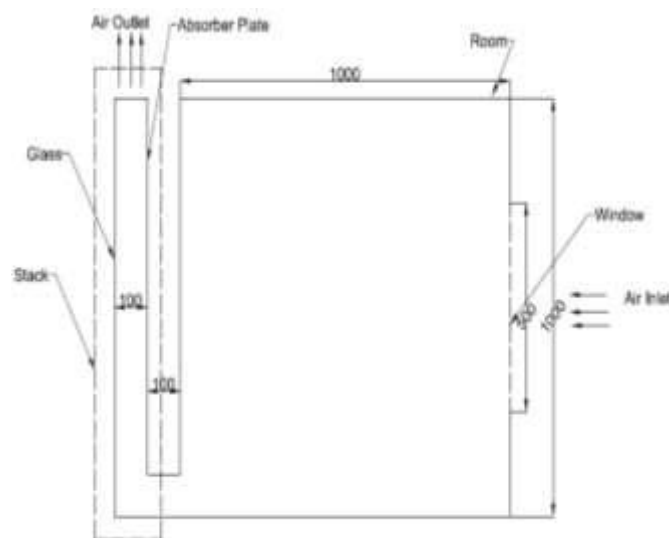
Fig.4.1: Line Diagram of Vertical Solar Chimney
