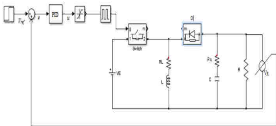
Fig. 2: The PID controller for Buck-Boost converter
