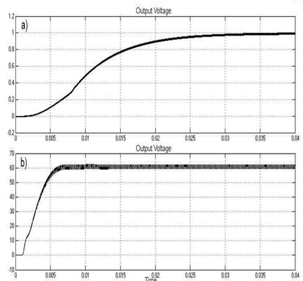
Fig. 8 The step response of the Buck-Boost converter with PID control: a) V_{ref} = 1 V , b) V_{ref} = 60 V
