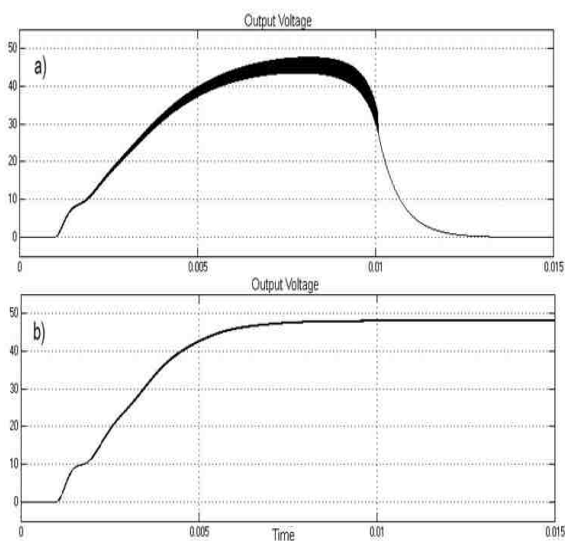
Fig. 9: The step response of the Buck-Boost converter with PID control: a) R = 12\Omega , b) R = 100\Omega
