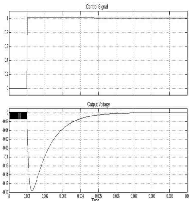
Fig. 4: Step response buck-boost converter with supercritical proportional gain
