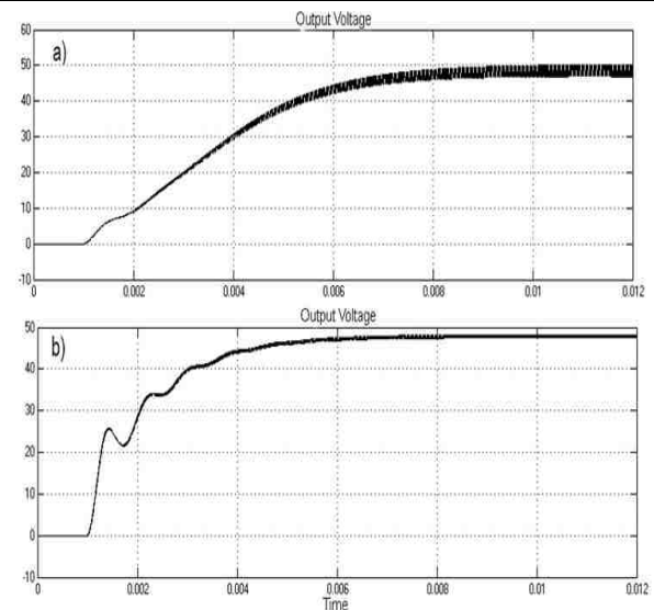
Fig.7: The step response of the Buck-Boost converter with PID control: a) V_E = 18.3 V , b) V_E = 96V
