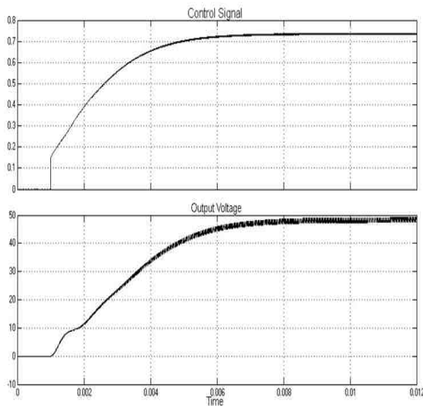
Fig. 6: Step response of the Buck-Boost converter with PID control.
