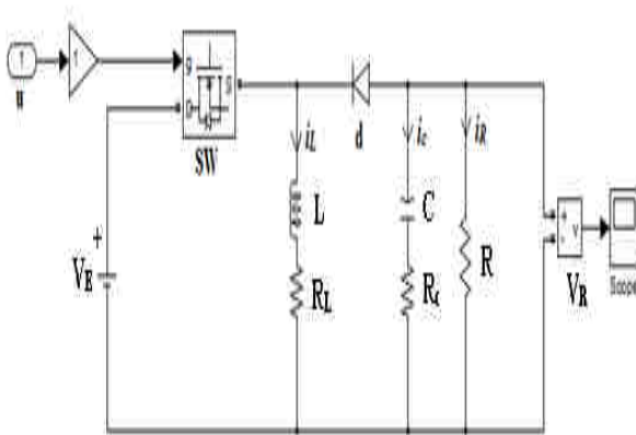
Fig.1:Buck-Boost circuit
