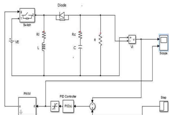
Fig. 3: The Simulink model of the buck-boost converter with PID controller.
