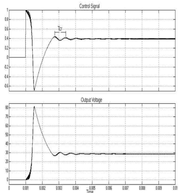
Fig. 5: Step response of the buck-boost converter with subcritical proportional gain.
