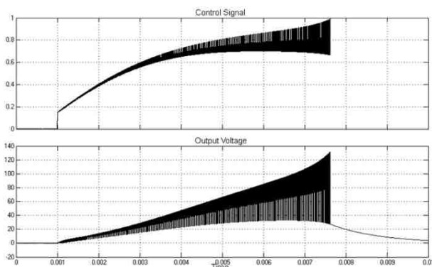
Fig. 10 : The step response of the Buck-Boost converter with great resistance in the branch capacitor ( R_C = 4\Omega ).
