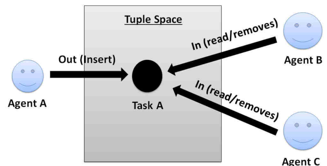
Fig.1: An abstract representation of the schedule tuple space
