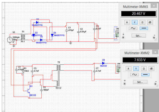
Fig.3: Circuit Simulation on Multisim Software
