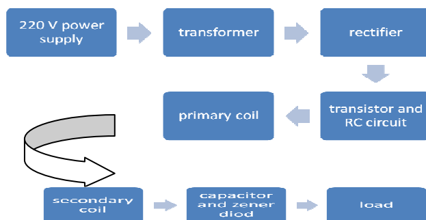
Fig.4: Block Diagram of Wireless Transmission
