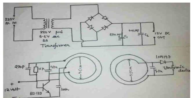
Fig.2: Circuit idea
