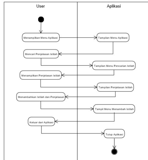
Gambar 3. Activity Diagram
