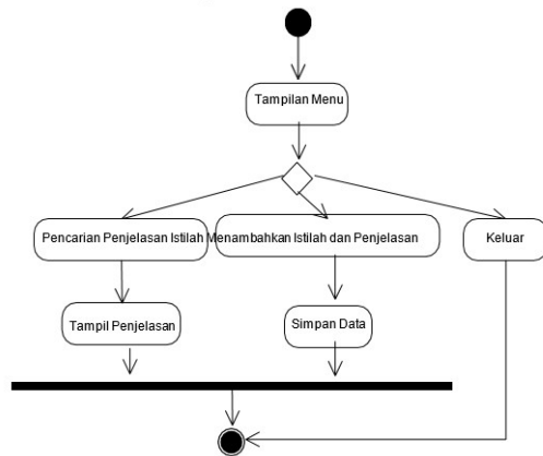
Gambar 5. State Diagram
