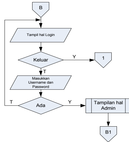
Gambar 3. Flowchart Login Admin
