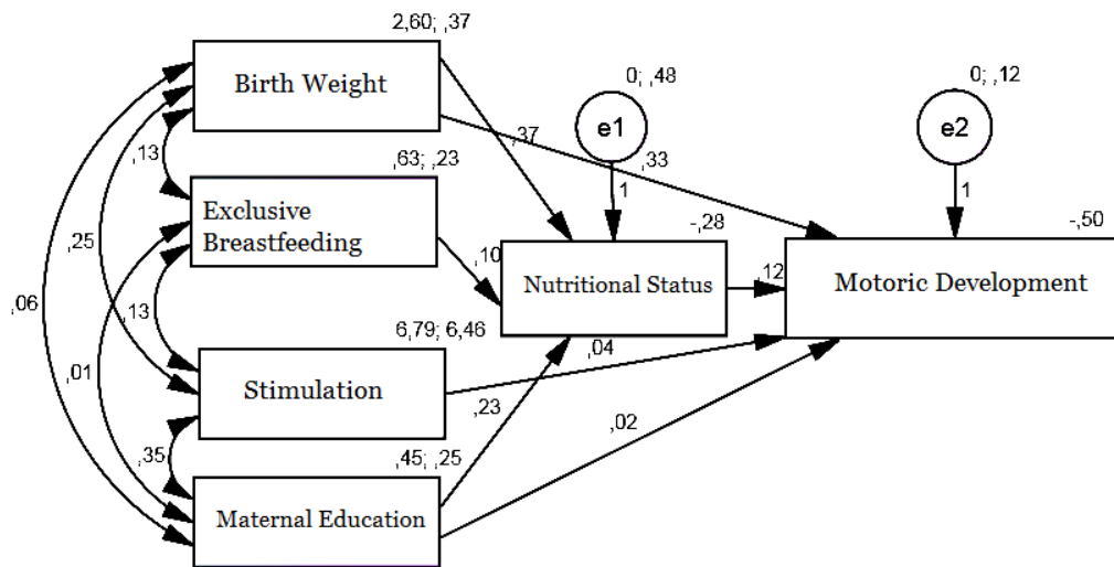
Picture 1. Structural model of unstandardized solution
