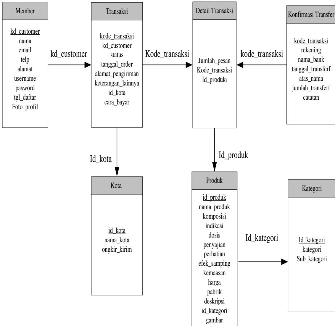
Gambar 7. Logical Record Structure Penjualan Online
