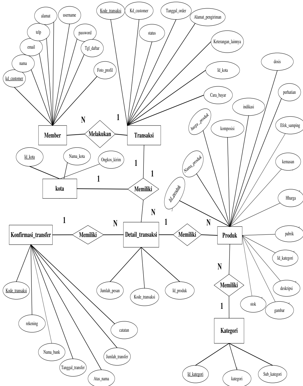
Gambar 6. Entity Relationship Diagram Penjualan Online
