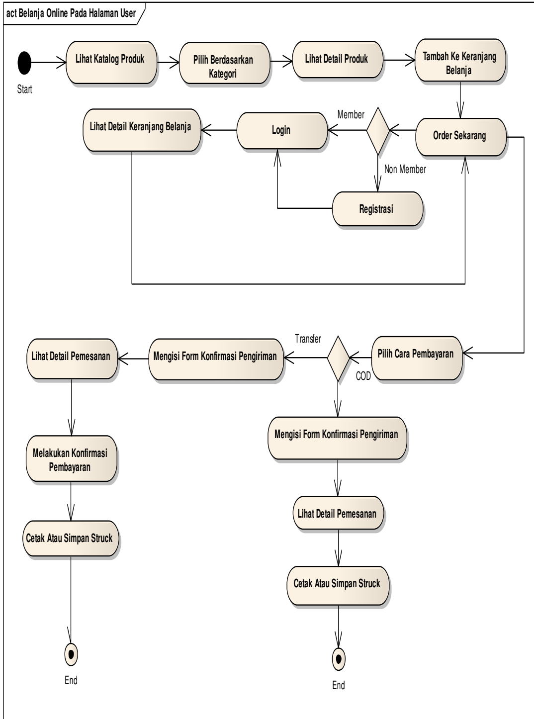
Gambar 5. Activity Diagram Belanja Online Halaman User
