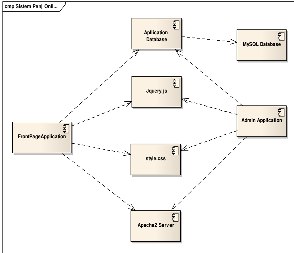
Gambar 8. Component Diagram Sistem Penjualan Online
