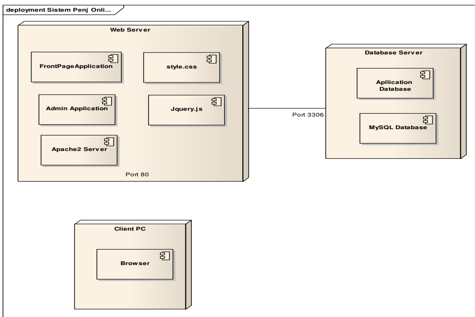
Gambar 9. Deployment Diagram Sistem Penjualan Online
