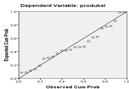
Gambar 3 : Digram Probabilitas
