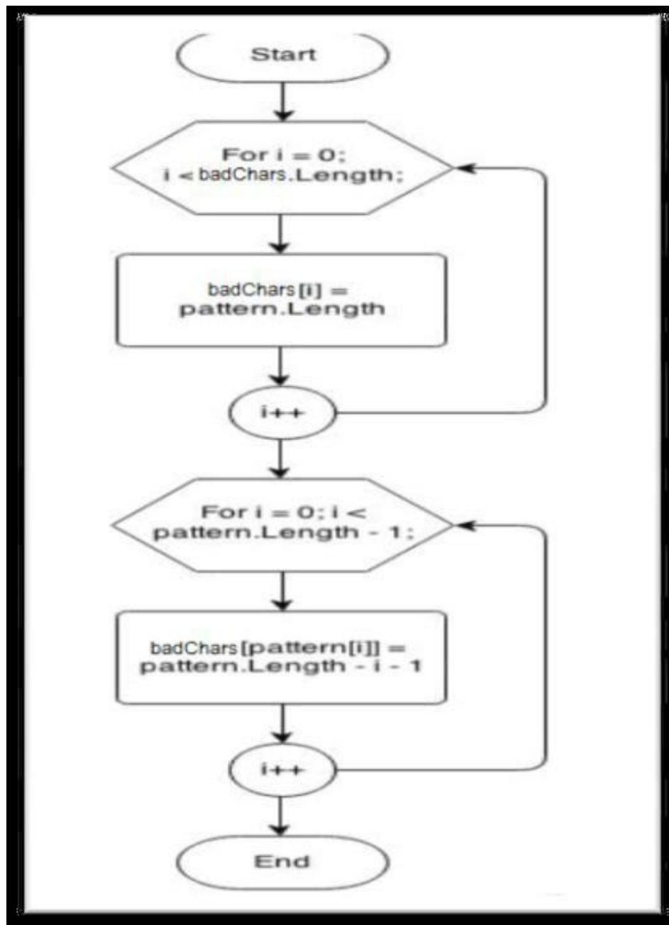
Gambar 5 Algoritma Boyer Moore
