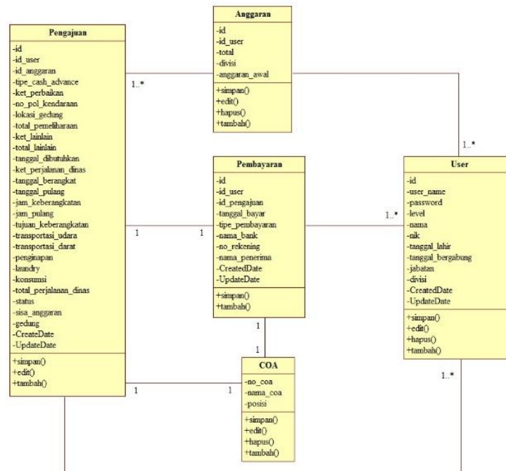
Gambar 7 Class Diagram
