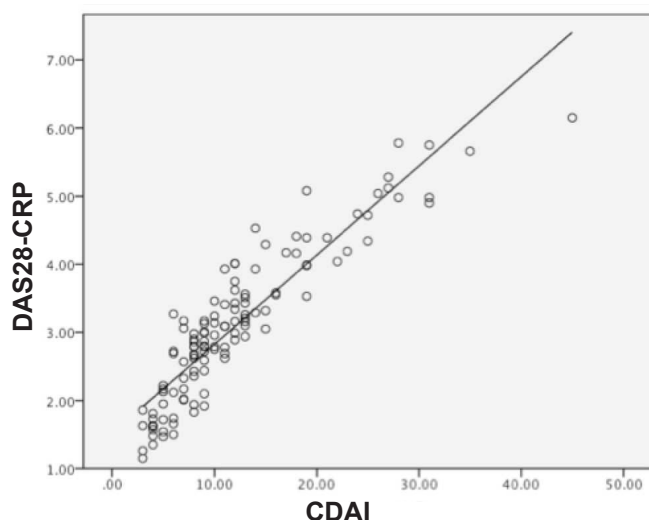
Figure 1. Correlation Plot of CDAI and DAS28-CRP
