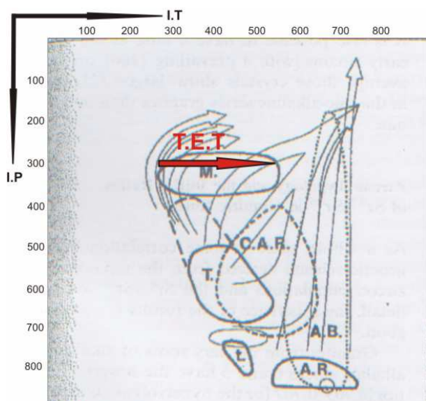
Gambar 6. Distribusi Typologi Berdasarkan Populasi Mineral Zirkon (Pupin, 1980), Migmatite (M), calc-alkaline series rhyolites (C.A.R), tonalites (T), alkaline basalts (A.B.), tracyandesites (t).
