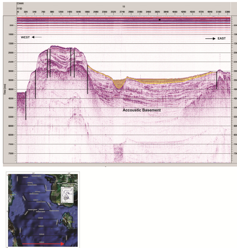
Figure 6. Seismic line 1 from west to east.
