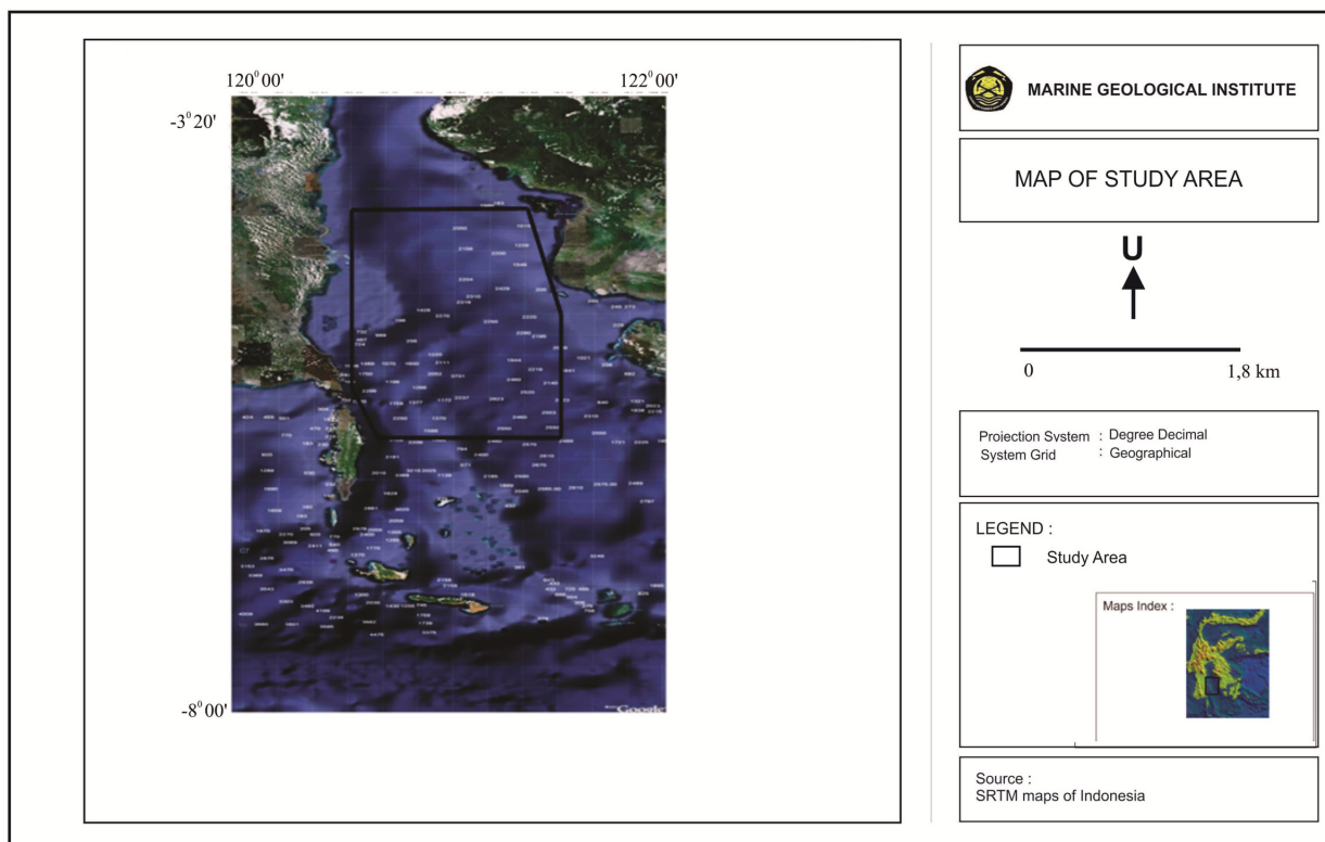
Figure 1. The study area of Bone Basin
