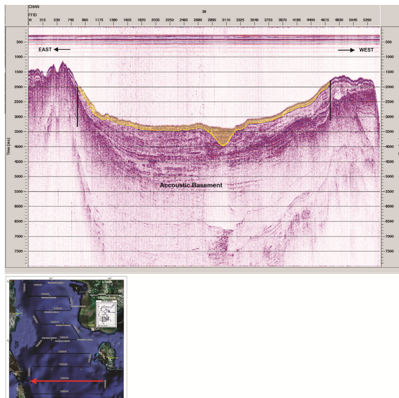
Figure 7. Sectional seismic reflection line 3 from east to west
