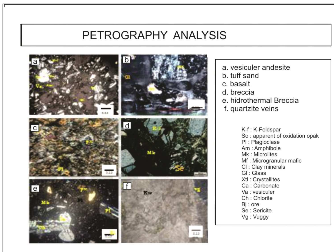
Figure 5. Petrography Analysis
