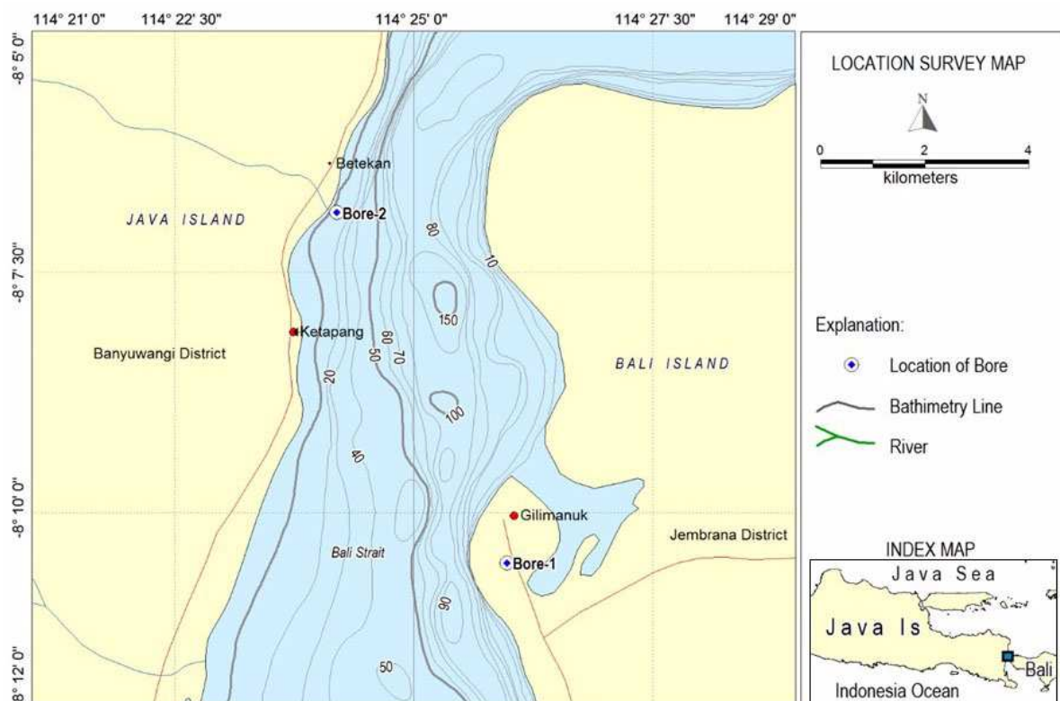
Figure 1. Location of bore holes and Bathymetry
