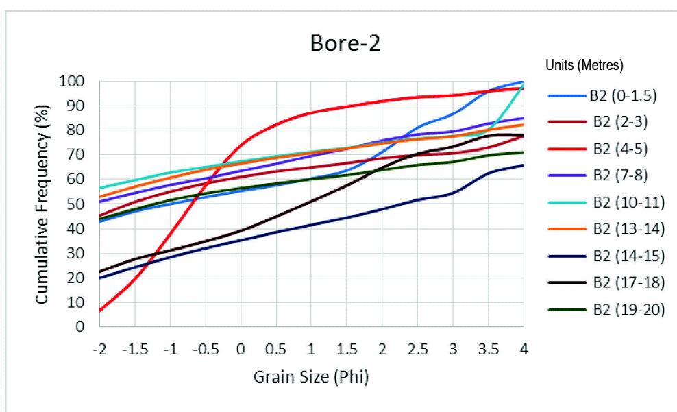
Figure 6. The relationship pattern between grain size (phi) and cumulative frequency (%) in Bore-2.
