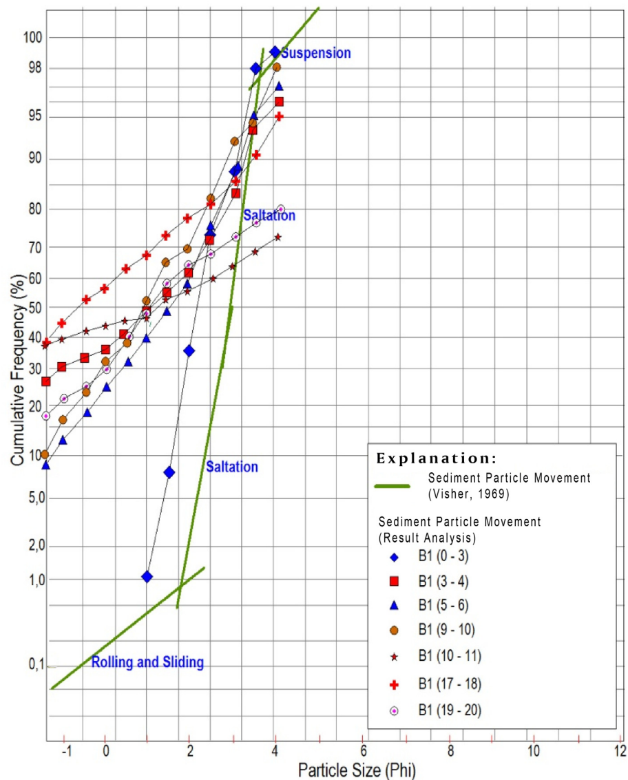
Figure 7. Analysis model of sediment movement on seven samples of Bore-1 (Visher, 1969; in Usman and Silalahi, 2009).
