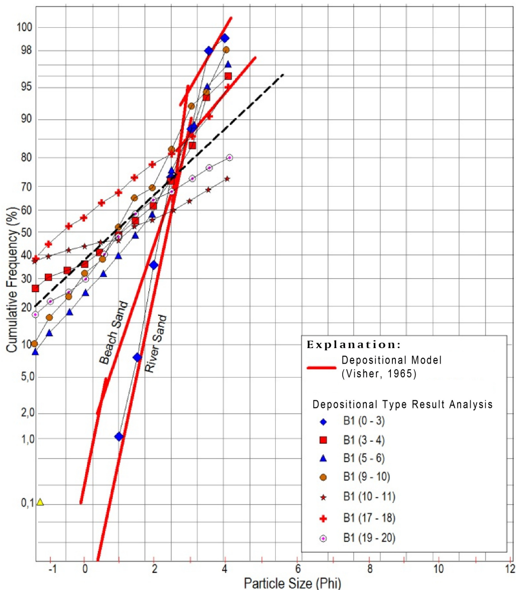
Figure 9. The model of depositional environment of sediment at Bore-1 according to Visher, 1965; in Usman and Silalahi, 2009.
