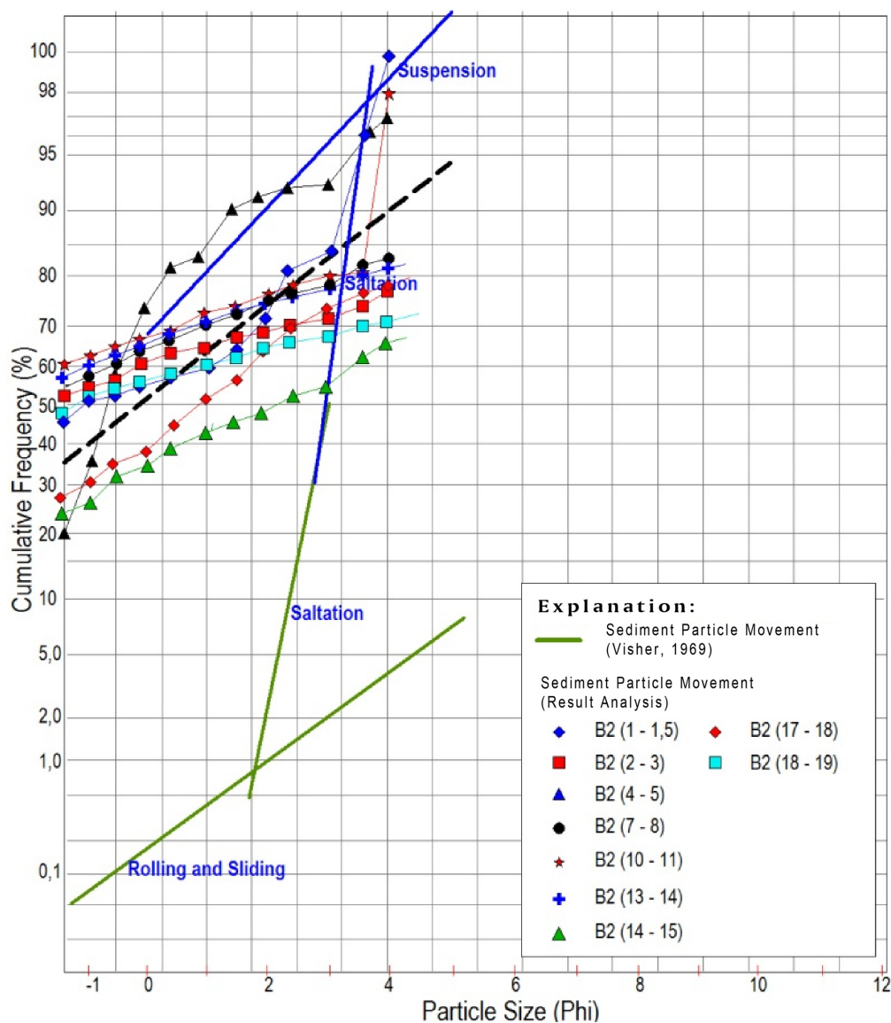
Figure 8. Analysis model of sediment movement on nine samples of Bore-2 (Visher, 1969; in Usman and Silalahi, 2009).
