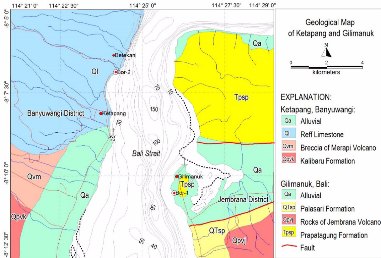
Figure 2. Geological map of study area and it's surroundings (modification from Sidarto et al, 1993 and Purbo-Hadiwidjojo et al, 1998; in Usman, 2007).
