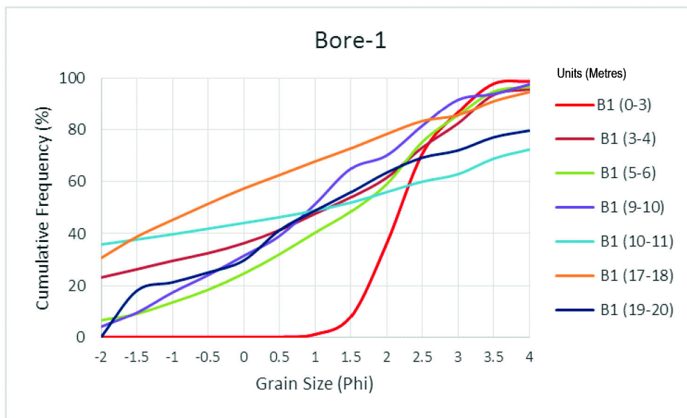
Figure 5. The relationship pattern between grain size (phi) and cumulative frequency (%) in Bore-1.
