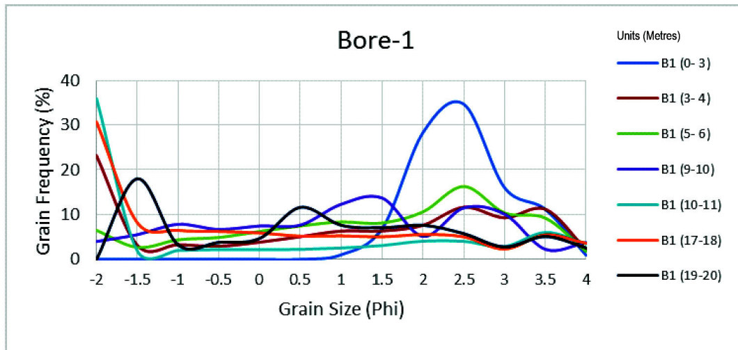
Figure 3. The pattern of uniformity frequency percentage of grains based on the relationship between grain size (phi) and the percentage of grains (%) in the sediment sample of Bor-1.
