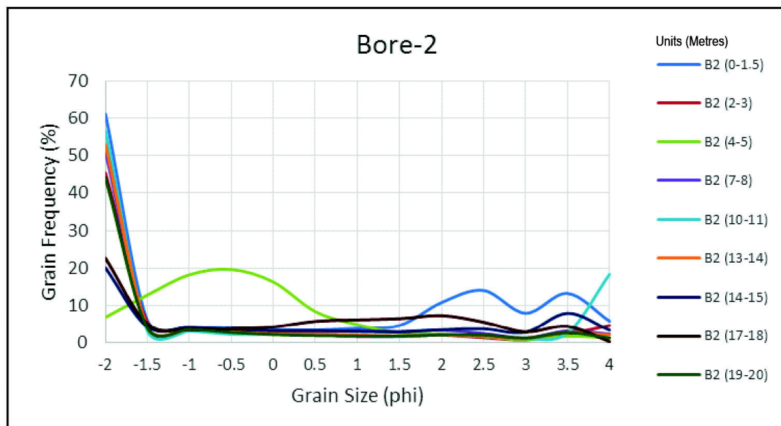
Figure 4. The pattern of uniformity frequency percentage of grains based on the relationship between grain size (phi) and the percentage of grains (%) in the sediment sample of Bor-2.
