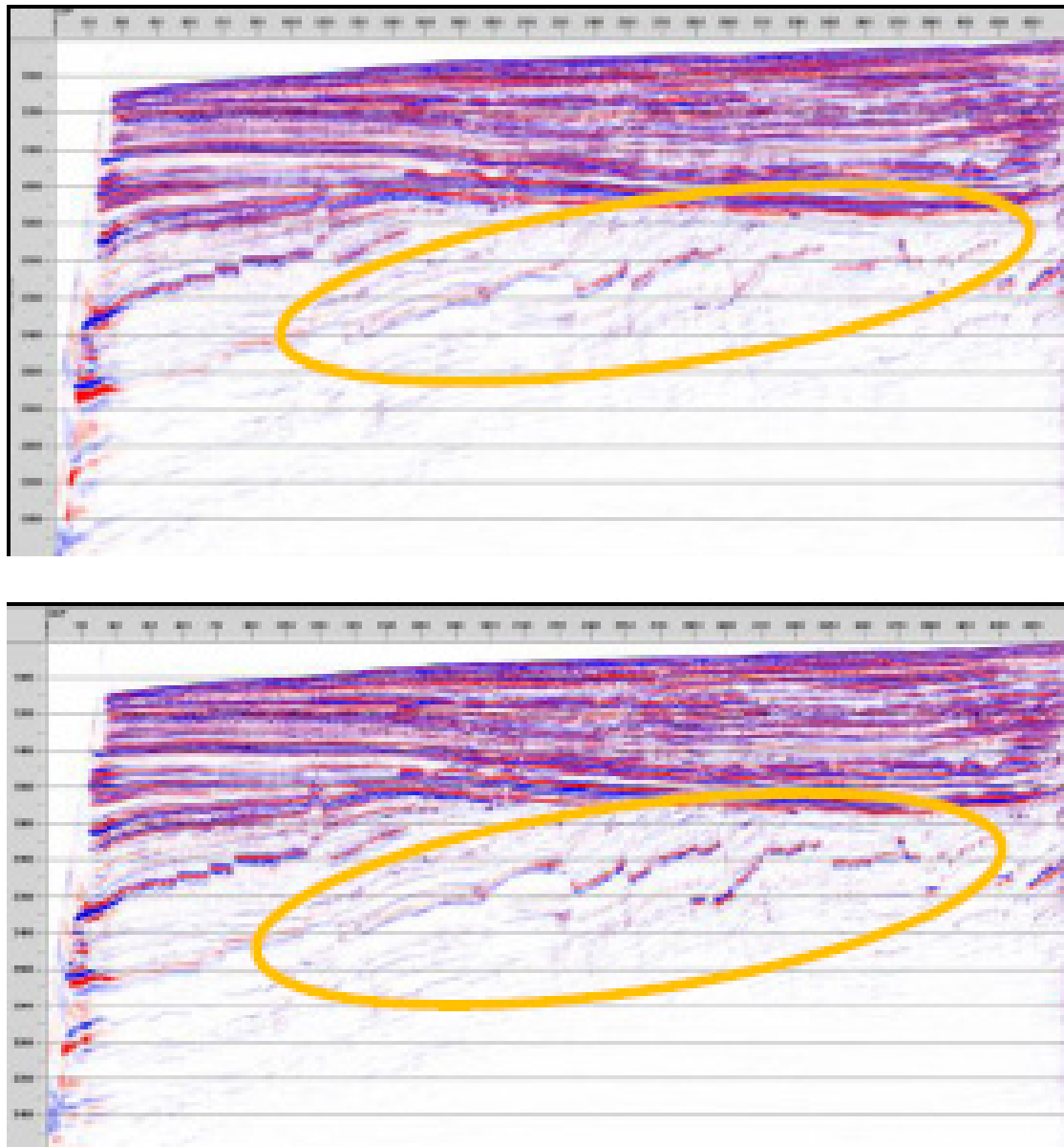
Figure 10. Comparison between depth-migrated seismic section PSDM using Dix-transformation and coherency inversion (top) and tomography (below)
